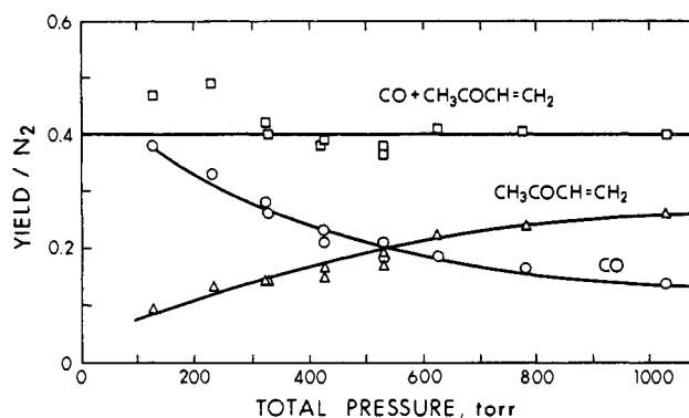
Figure 1. Yield ratios for CO/N 2 (O), CH 3 COCH=CH 2 /N 2 (Δ), and their sums (□), as a function of total pressure, from the reaction of O( 3 P) atom with dimethylacetylene.
